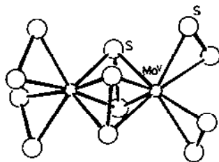
Fig. 4. Structure of the [\text{Mo}_2(\text{S}_2)_6]^{2-} ion.
