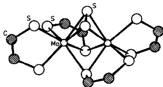
Fig. 6. Structure of \text{Mo}_2(\text{S}_2)(\text{S}_2\text{C}_2\text{Ph}_2)_4 ; phenyl groups omitted for clarity.
