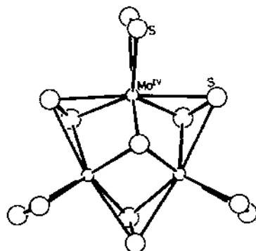
Fig. 5. Structure of the [\text{Mo}_3\text{S}(\text{S}_2)_6]^{2-} ion.
